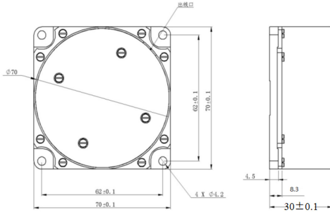
Graph 2 Outline dimensions of G-F70HA
