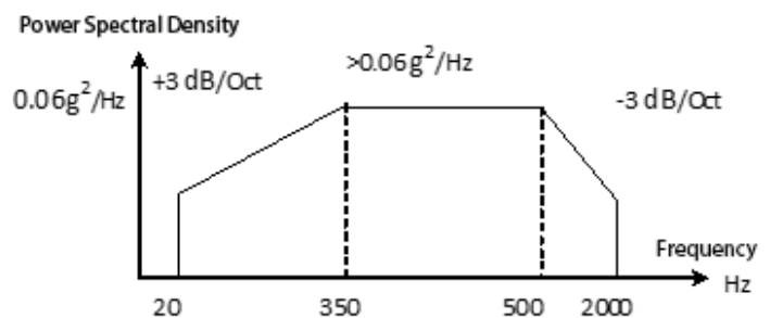
Figure 1 Vibration spectrogram
